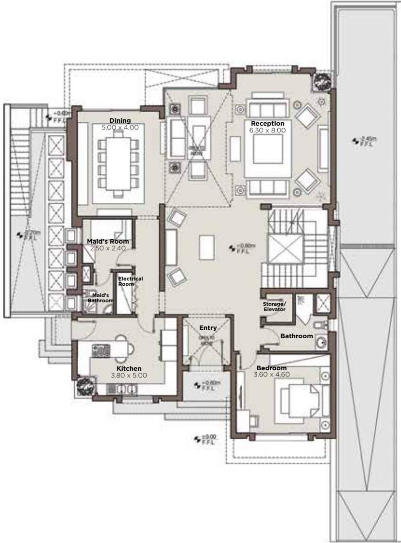
GROUND FLOOR 207 m 2
